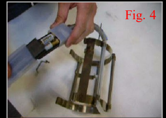
Fig.3 and 4. Lift up the whole unit and pull the hood gently backwards to open the battery compartment
